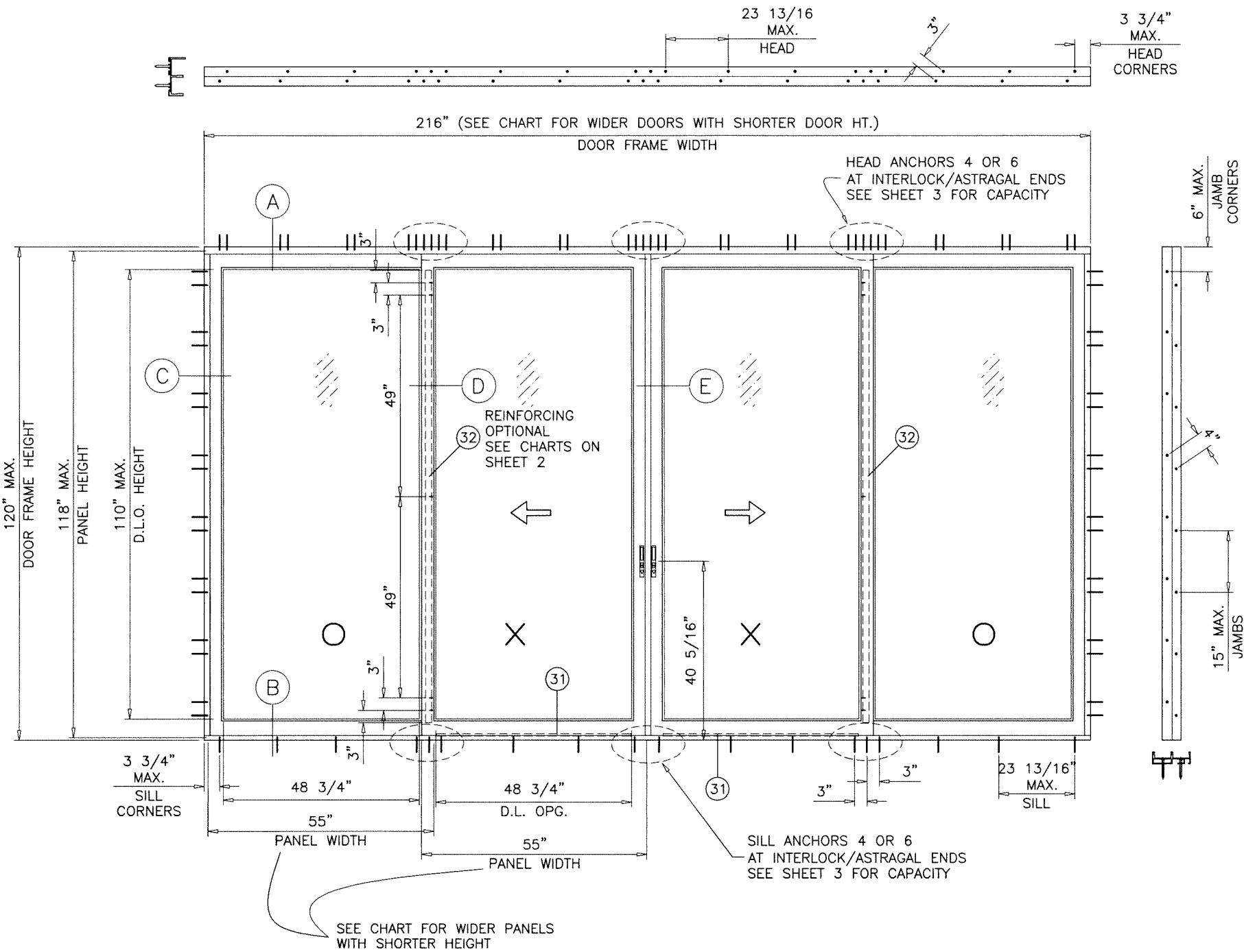
TYPICAL ELEVATION TESTED UNIT
