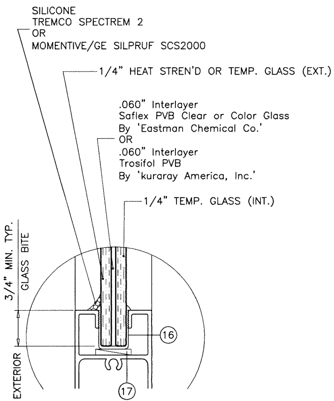
GLAZING DETAIL 9/16" OVERALL LAM. GLASS
